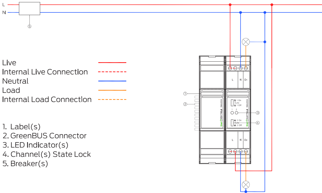
Figure 4: Wiring Diagram
