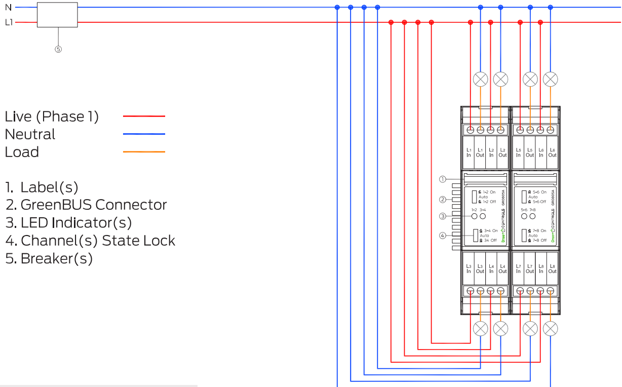
Figure 4: Wiring Diagram
