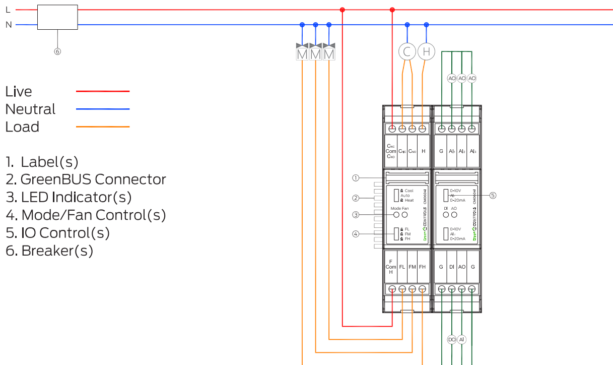
Figure 4: Wiring Diagram
