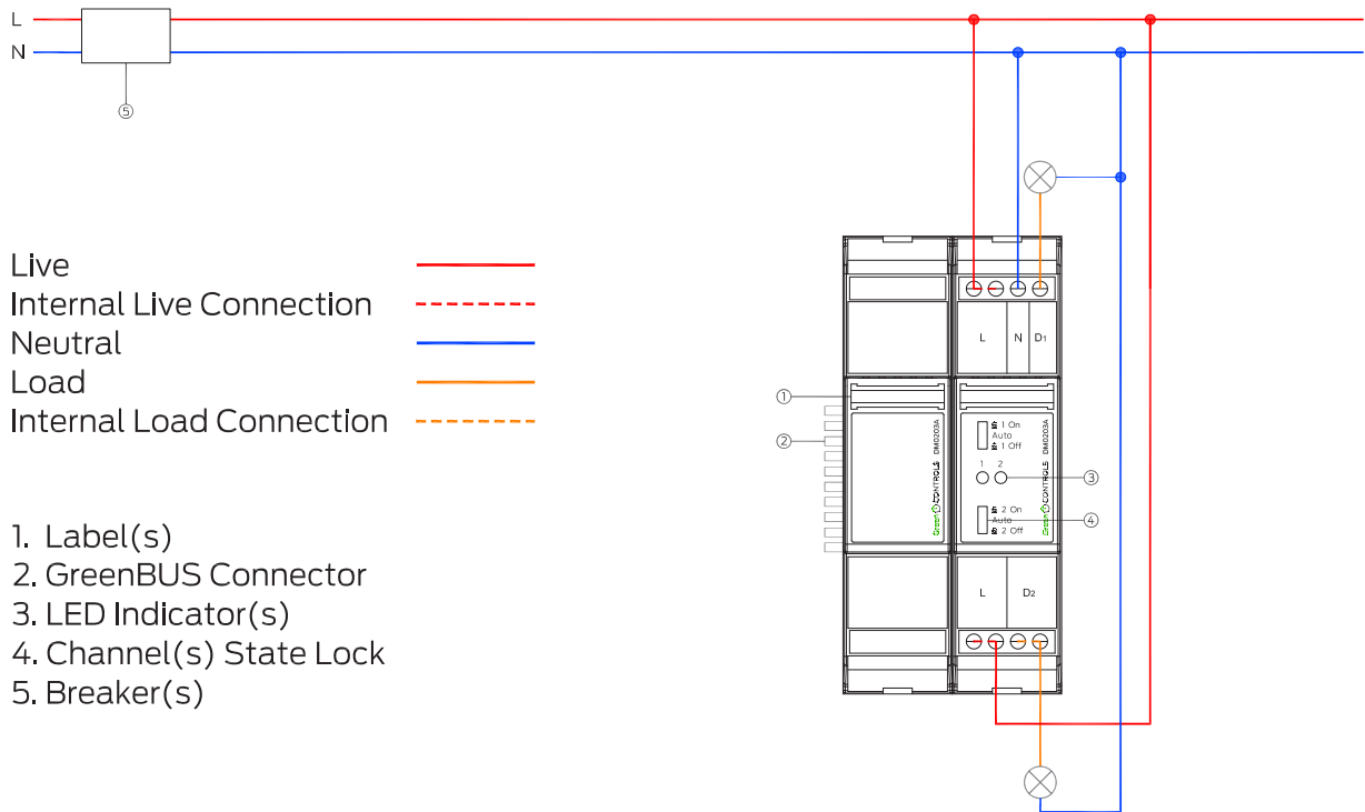
Figure 4: Wiring Diagram
