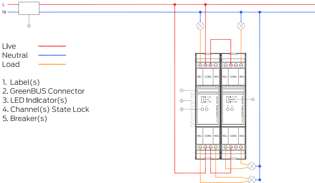
Figure 4: Wiring Diagram
