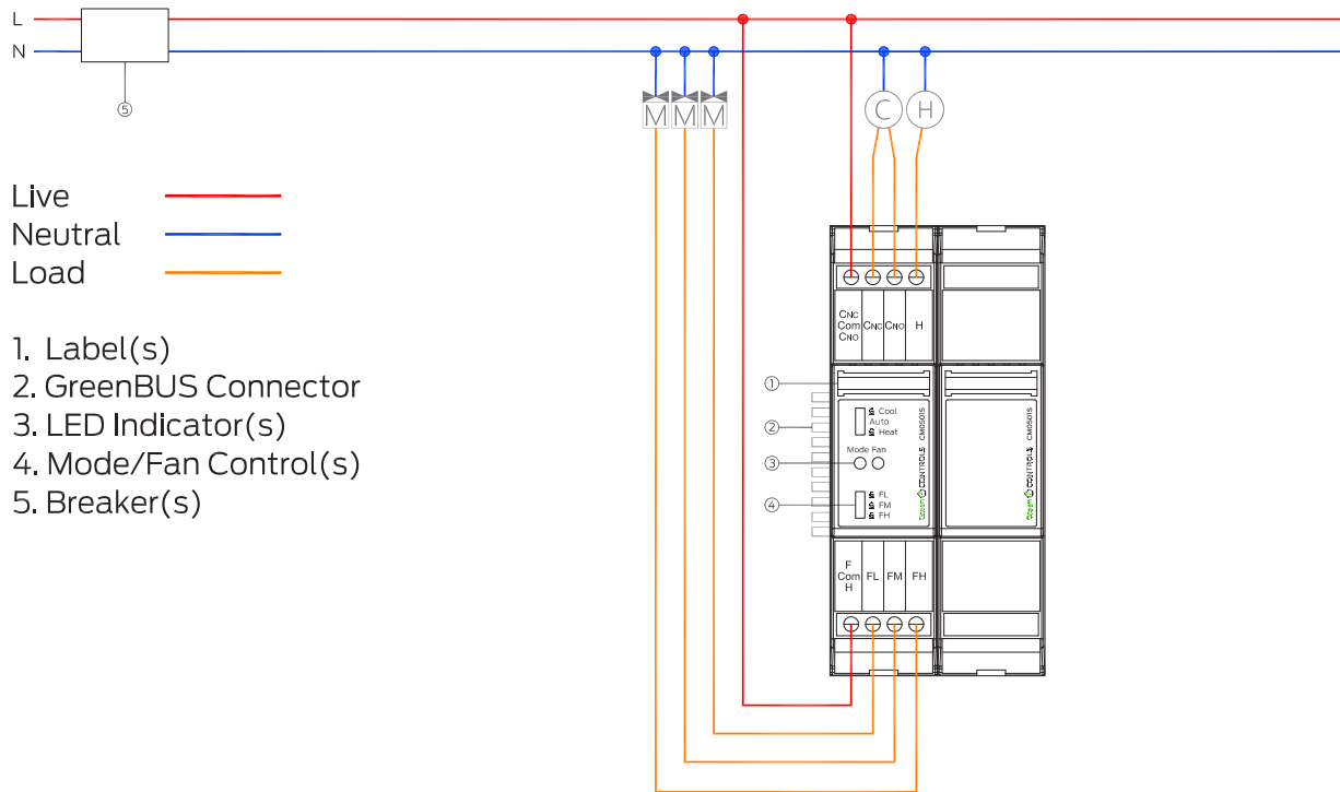
Figure 4: Wiring Diagram
